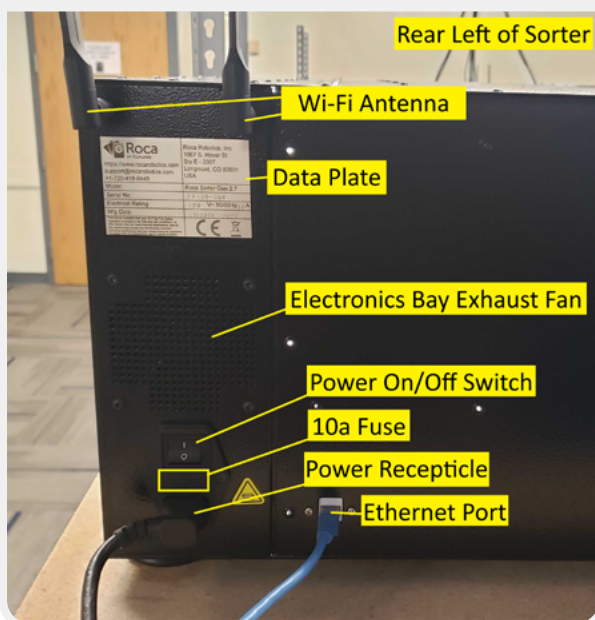
Rear View (LH)
