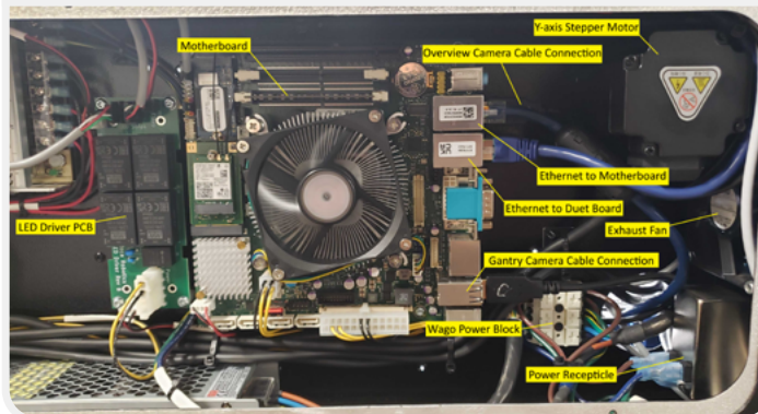
Rear of Electronics Bay
