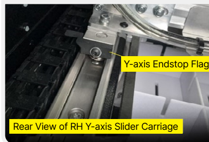
Gantry Assembly (RH)
