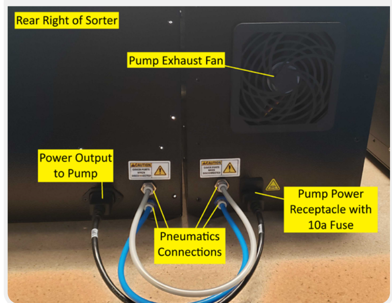
Rear View (RH)
